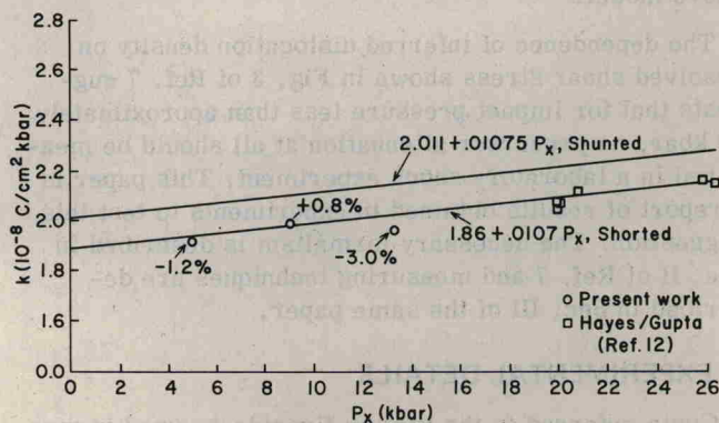
FIG. 1. Effects of pressure on the piezoelectric constants of quartz gauges.
